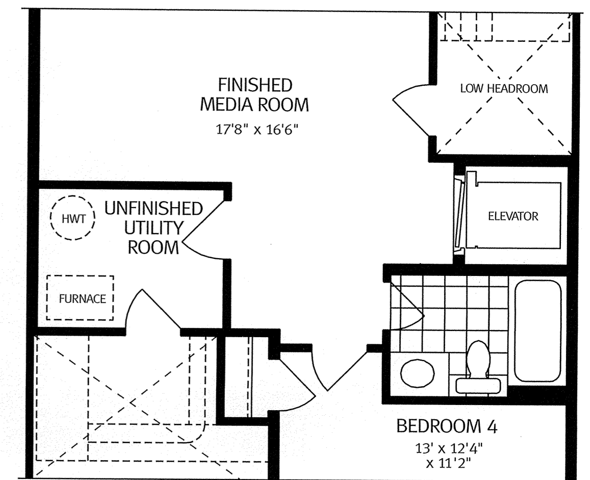
PART. GROUND FLOOR PLAN OPTIONAL ELEVATOR LAYOUT
